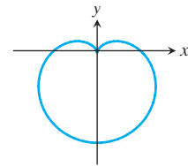
44. Kardiod
